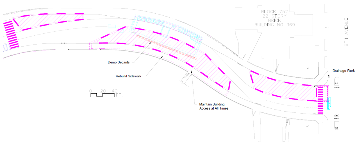
Stage 2 - Installing/Rerouting Utility Lines, Secant Piles
