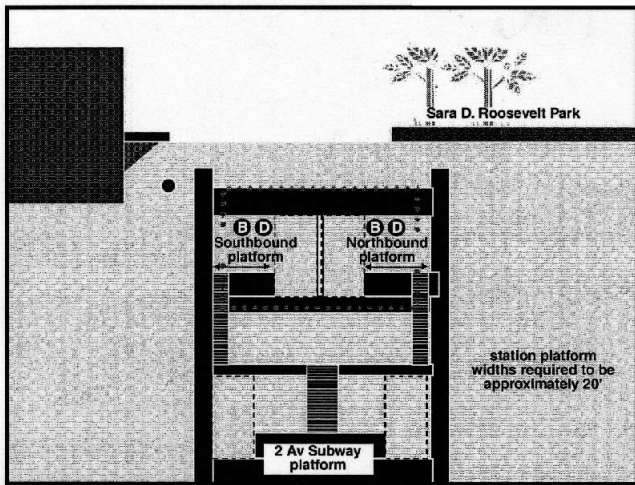
Reconstructed Grand St Station with new Second Avenue Subway platform below - profile view Sketch for conceptual purposes only - not to scale
