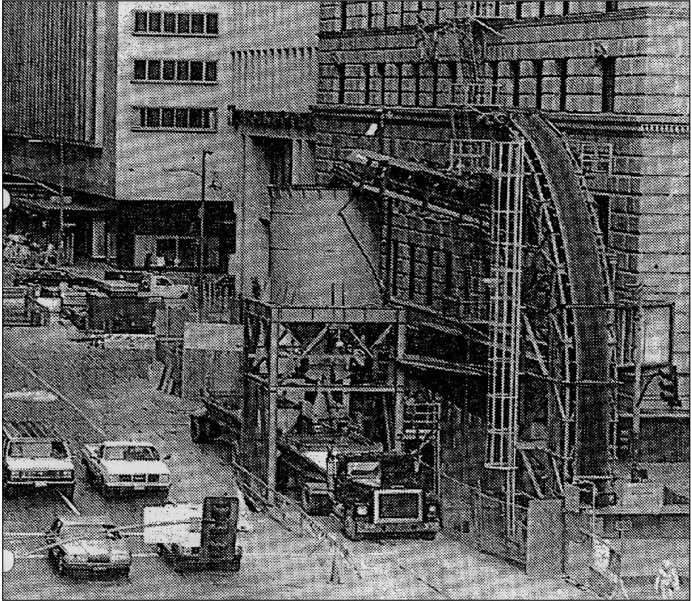
Example of a muck hopper used to store spoils removed from tunnels
